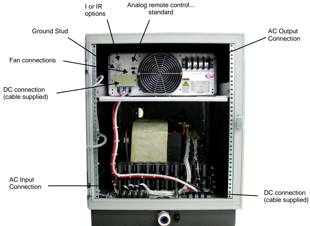
Rear View
